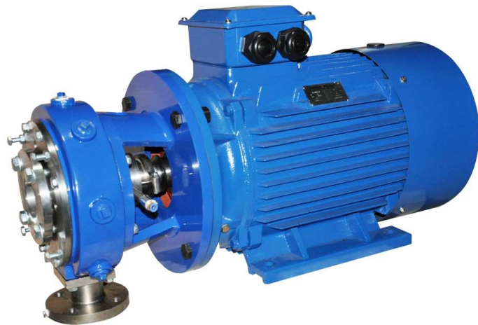
胶体磨定转子 ( Rotor and Stator ) 沥青胶体磨 ( Bitumen emulsion mill )
